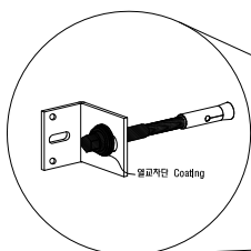
T.B. FASTENER SINGLE ANCHOR TYPE BASIC
