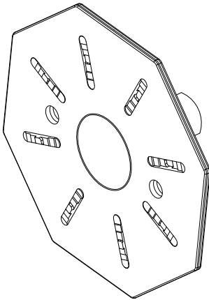
T.B FASTENER SINGLE ANCHOR TYPE TURNCAP
